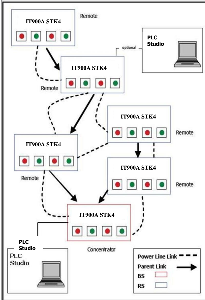
Figure 7: Basic NL Setup
