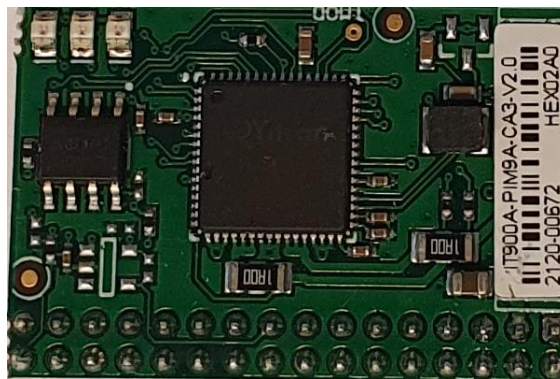
Figure 3: IT900A PIM
